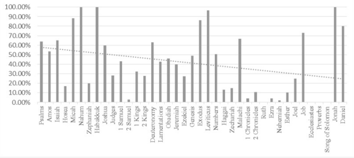
Percentage of Character Instances with MCI Features (Chronological w/ Trend Line)
